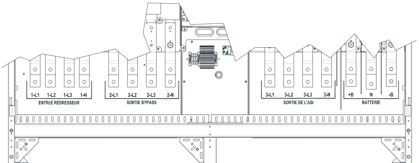
Illustration 7A – Borniers KEOR HPE 600 kVA
