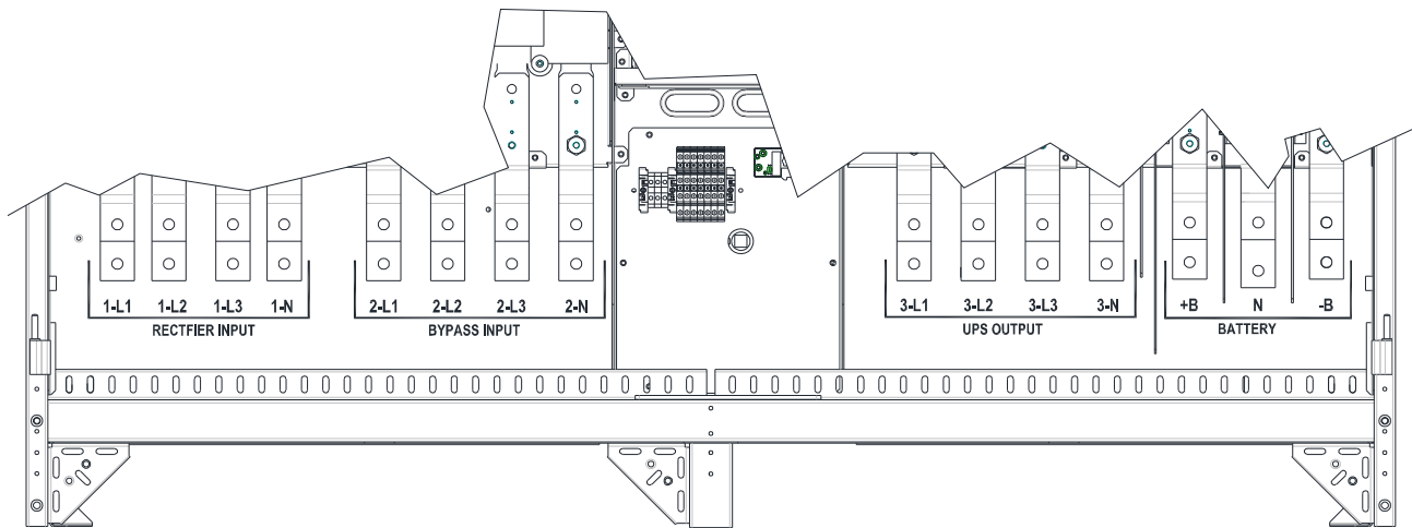
Picture 7A – Terminal board KEOR HPE 600 kVA
