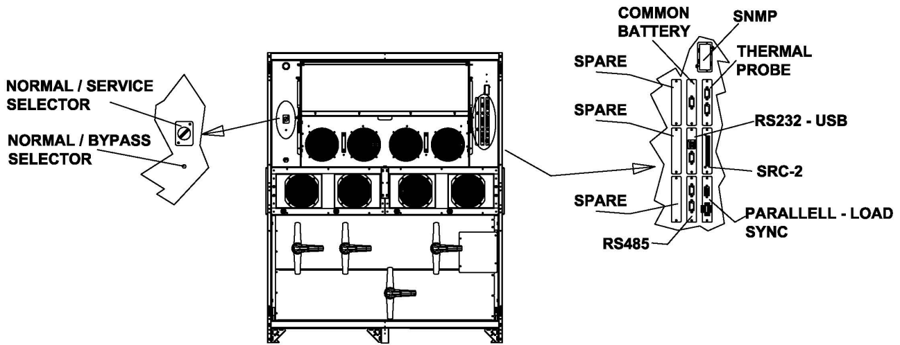
Picture 9A – Position of the serial interfaces of KEOR HPE 600 kVA
