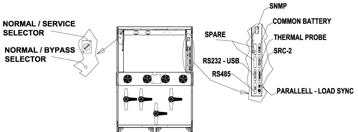
Picture 9 – Position of the serial interfaces of KEOR HPE 400-500 kVA
