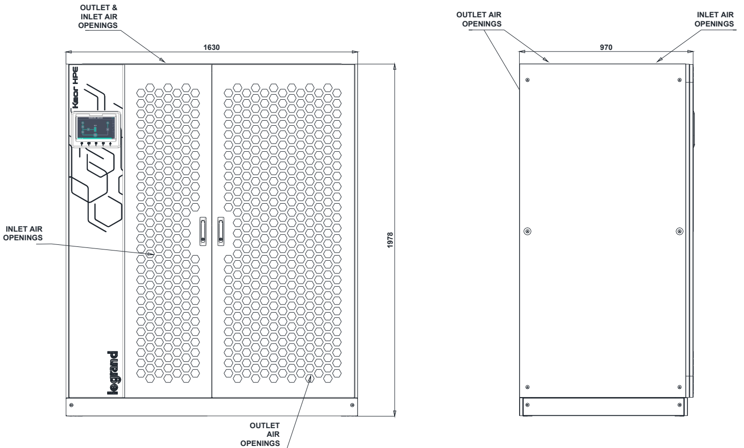
Picture 4A – Overall dimensions KEOR HPE 600 kVA
